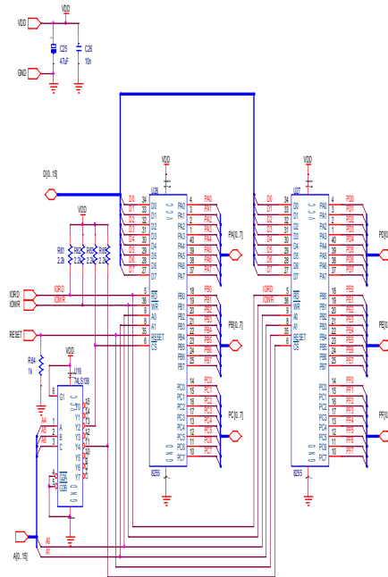
Fig. 2(a) Circuit Diagram of Simple Input/ Output
