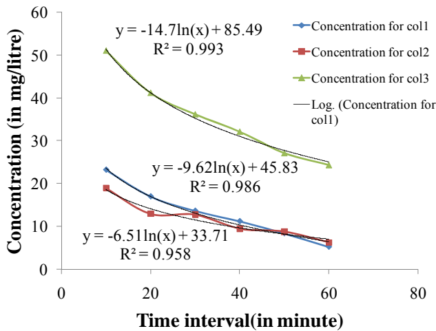
Fig. 6 Plot of Concentration vs time graph for calcium at flow rate 50 ml/sec for 3 columns. Height ratio H2/H1 for 3 columns are= 8/6, 5/15, 3/18
