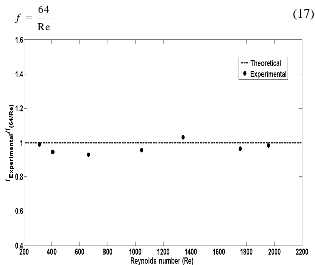
Fig. 6 Ratio of experimental friction factor to theoretical prediction for distilled water versus Re number
