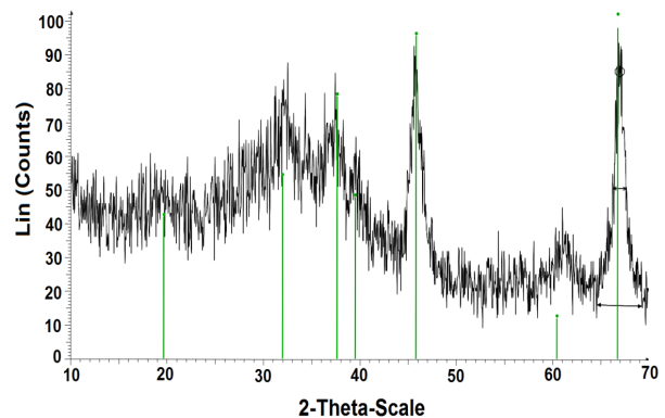
Fig. 2 XRD image of the \text{Al}_2\text{O}_3 nanoparticles
