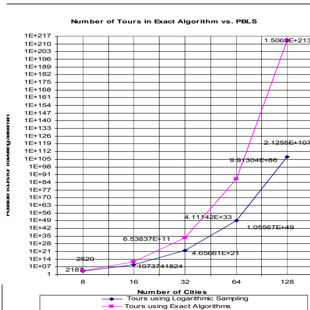
Fig. 3 Graph illustrating the comparison of pbls and exact algorithms with respect to number of tours
