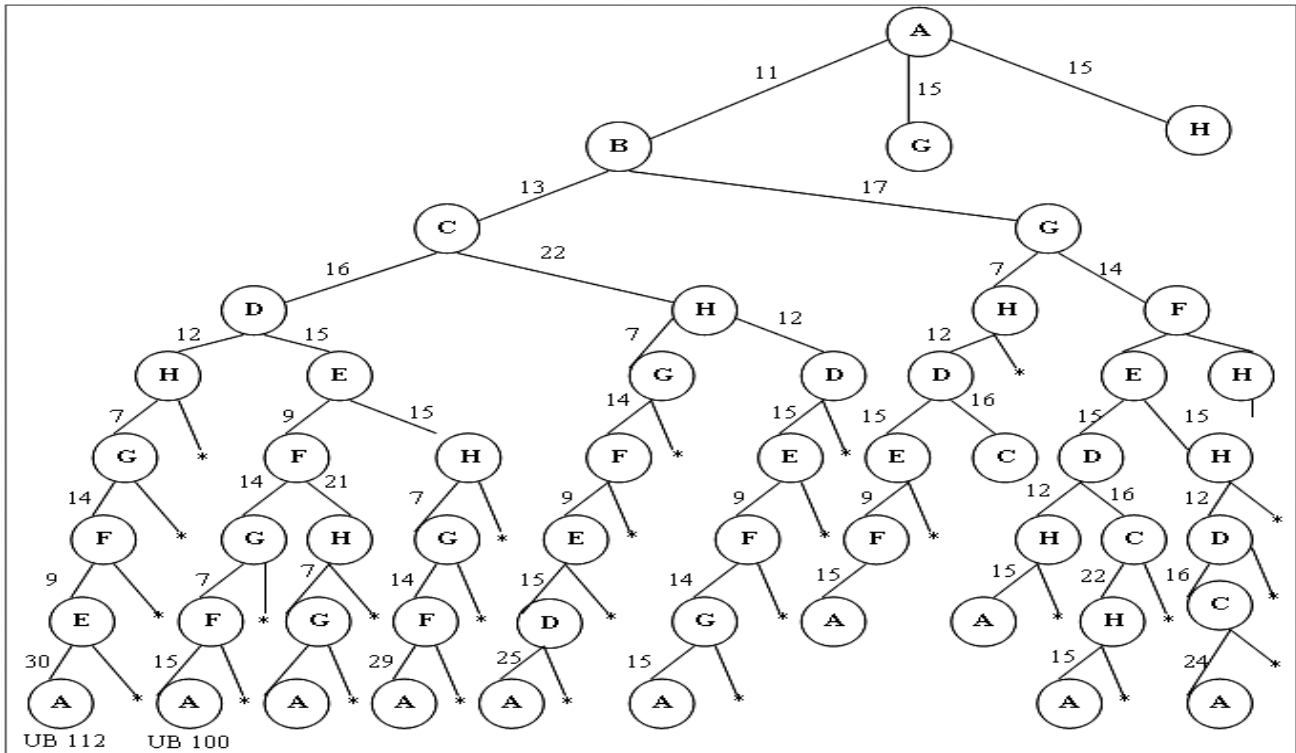
Fig. 2 Search process on the matrix in table ii. All possible branches will be explored. Here only branch 'b' of 'a' is shown. Upper bound is maintained after the completion of each successful path.
