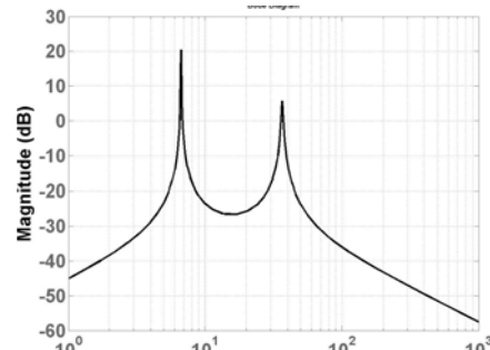
Fig. 19 Bode plots for model 1 of system 2 (fixed end)
