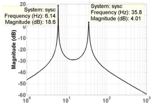
Fig. 20 Bode plots for model 1 of system 3 (fixed end)
