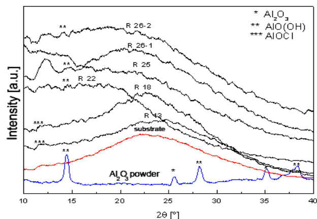
Fig. 2 XRD spectra for Al 2 O 3 films deposited onto glass substrate from AlCl 3 solutions in water- ethanol mixture
