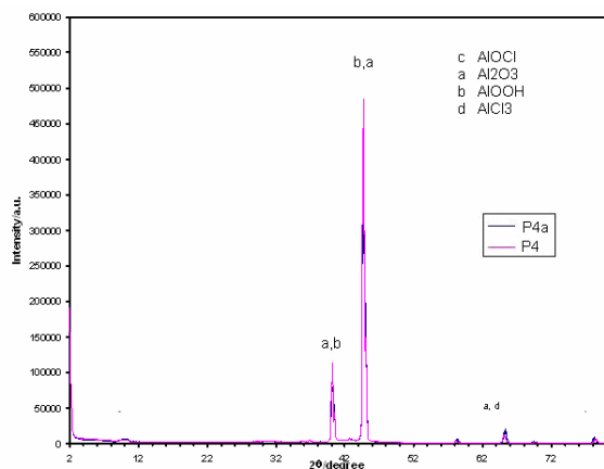
Fig. 1 XRD spectra for 2 films deposited onto aluminum substrate from aqueous Al 2 O 3 solutions
