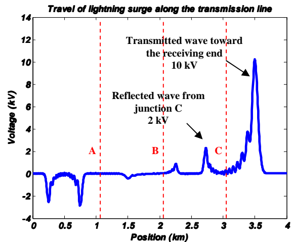
Fig. 10 Transmitted and reflected waves at junction C
