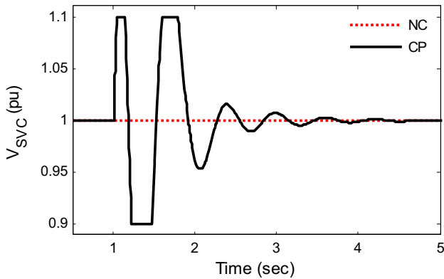
Fig. 9. SVC reference voltage signal for Case-I
