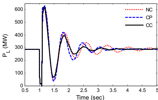
Fig. 7. Tie-line power flow response for Case-I
