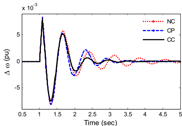
Fig. 6. Speed deviation response for Case-I
