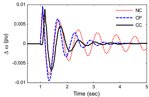
Fig. 13. Speed deviation response for Case-III
