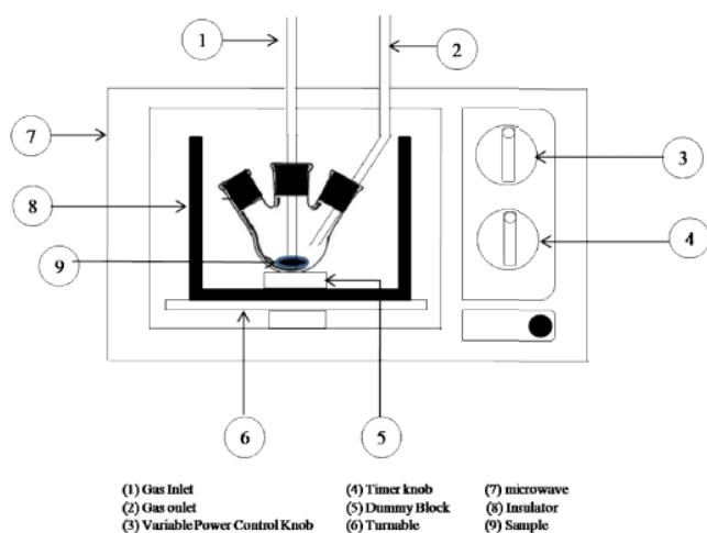
Fig. 1 The schematic diagram of modified microwave oven
