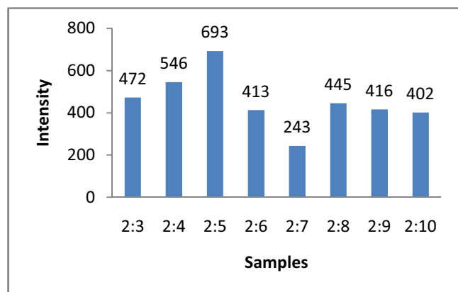
Fig. 4 Peak analysis at 23.3 ° for orthorhombic MoO 3
