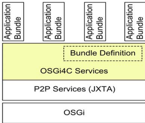
Fig. 3 OSGi4C Architecture
