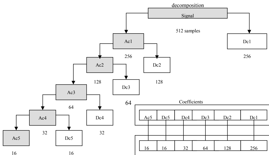
Fig. 1 Example of Wavelets coefficients calculation
