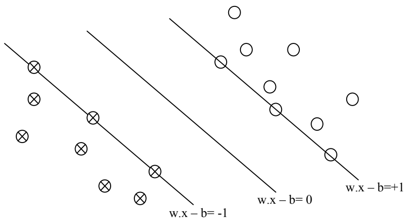
Fig. 2 The optimal separating hyperplane is located at the medium of the two classes
