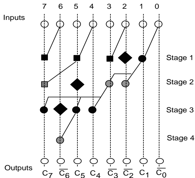
Fig. 1 Proposed 8-bit Parallel Prefix Adder
