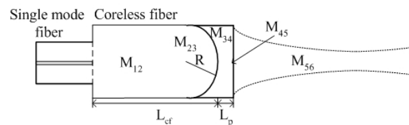
Fig. 1: The proposed fiber lens structure.
