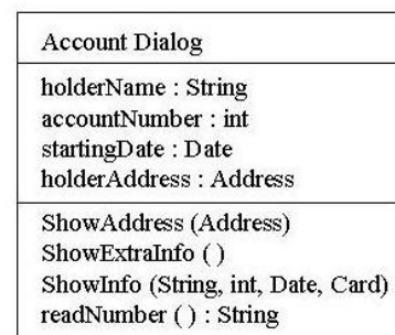
Fig. 1 UML class diagram for AccountDialog
