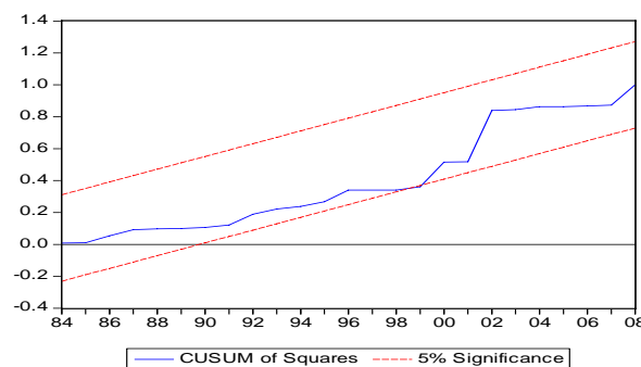
Fig. 4 Cumulative Sum of Squares of Recursive Residual (6)
