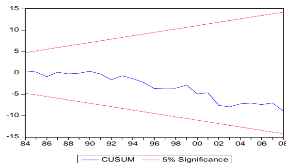
Fig. 3 Cumulative Sum of Recursive Residual on (6)
