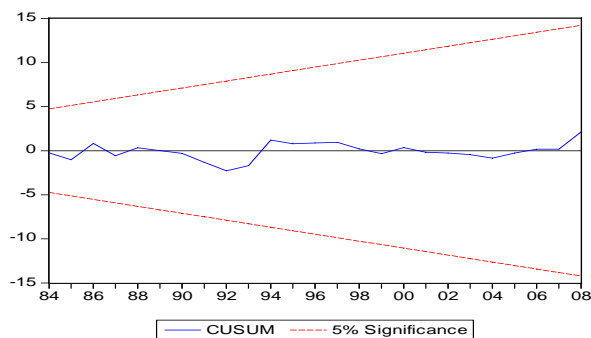
Fig. 1 Cumulative Sum of Recursive Residual on (4)
