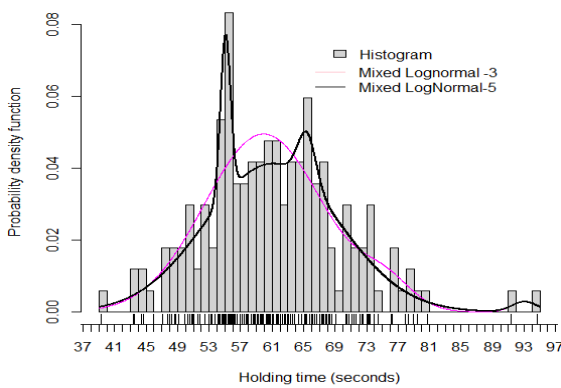
Fig. 3 Histogram of "103" data and its fitting pdf curves
