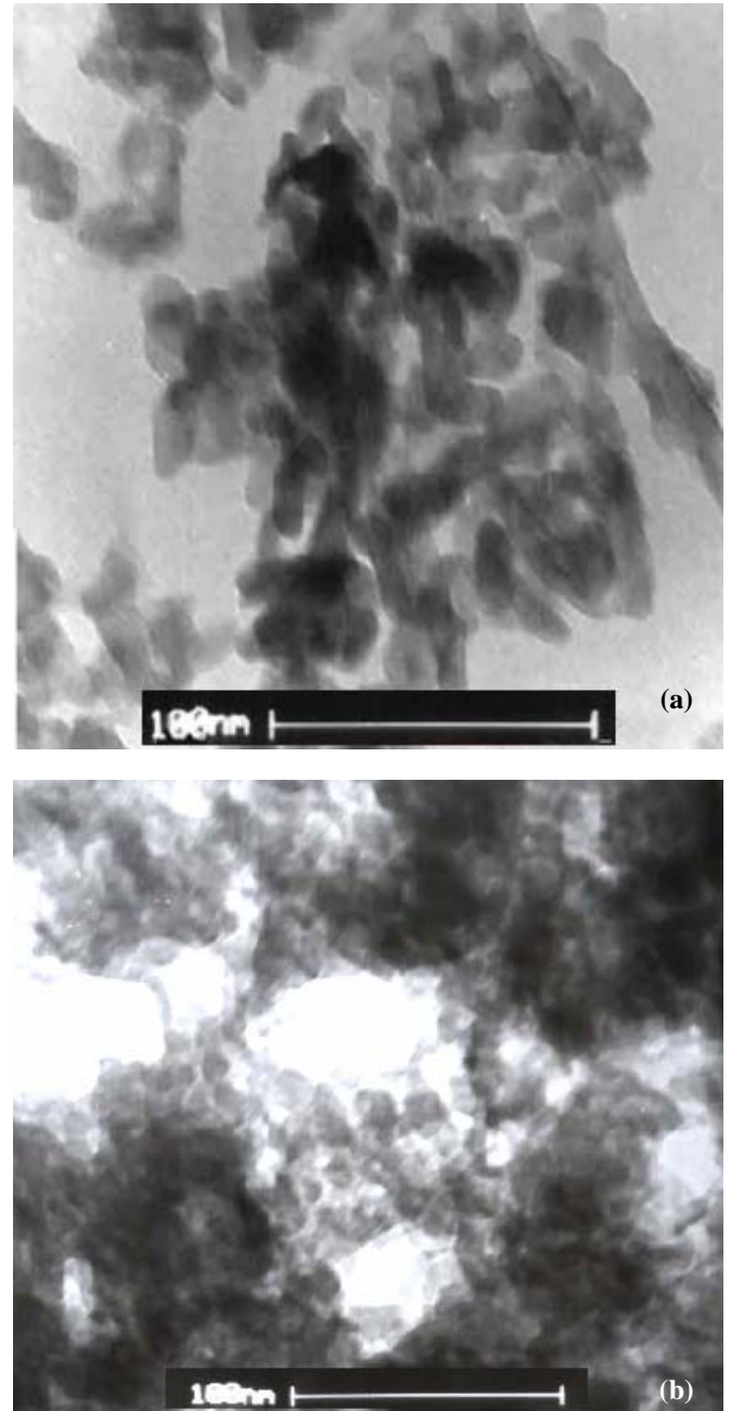
Fig.4. TEM micrographs of synthesized HAp (a) in the absence of polymer, and (b) in the presence of 5.6- 2.75 g gelatin-starch
