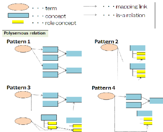
Fig.5 Mapping patterns for polysemous relation
