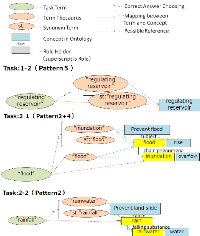
Fig. 11 Associations between task terms and concepts
