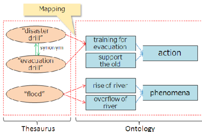
Fig.3 Overview of the mapping approach
