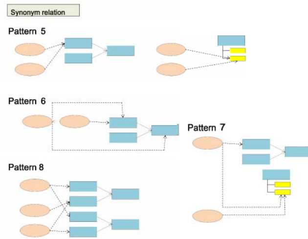
Fig. 6 Mapping patterns for synonymous relation
