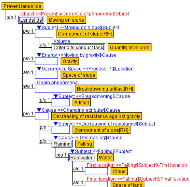
Fig. 10 Example of task concept definition
