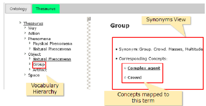
Fig. 13 Screen copy of Thesaurus viewer
