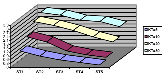
Fig. 1 Entropy comparison
