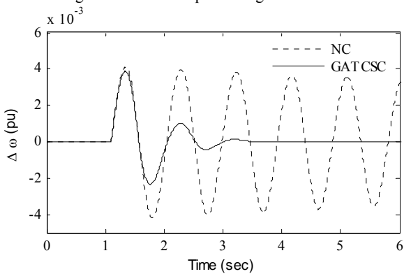
Fig. 19 Variation of speed deviation \Delta\omega : Case-2
