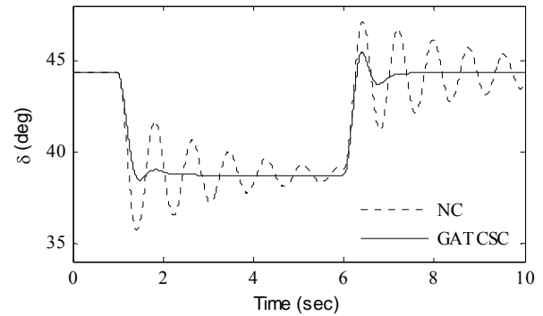
Fig. 27 Variation of power angle \delta : Case-3
