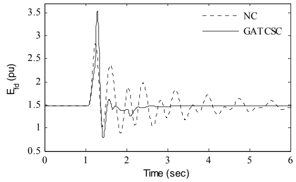
Fig. 13 Variation of voltage E_{fd} : Case-1
