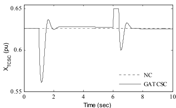
Fig. 31 Variation of X_{TCSC} : Case-3
