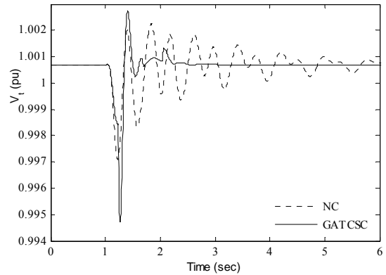
Fig. 14 Variation of terminal voltage V_t : Case-1
