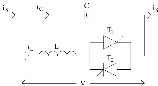
Fig. 2 Basic module of a TCSC
