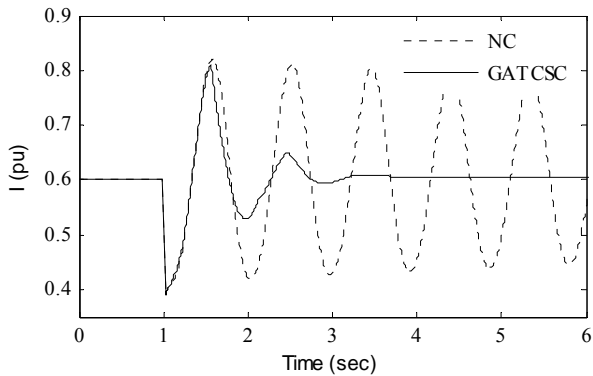
Fig. 25 Variation of line current I : Case-2
