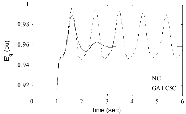
Fig. 22 Variation of voltage E'_q : Case-2
