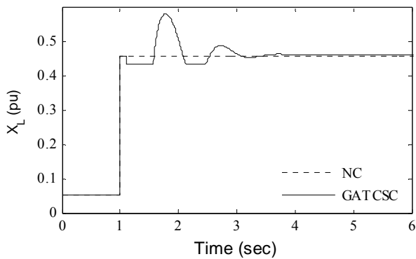
Fig. 26 Variation of transfer reactance X_L : Case-2
