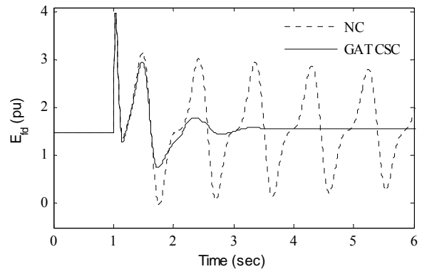
Fig. 23 Variation of voltage E_{fd} : Case-2
