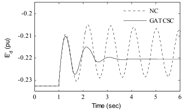
Fig. 21 Variation of voltage E'_d : Case-2
