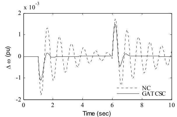
Fig. 28 Variation of speed deviation \Delta\omega : Case-3
