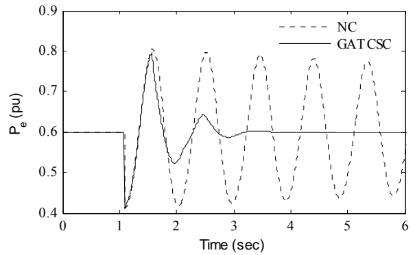
Fig. 20 Variation of electrical power P_e : Case-2
