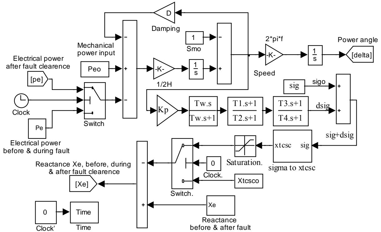
Fig. 5 SIMULINK model of SMIB with TCSC controller
