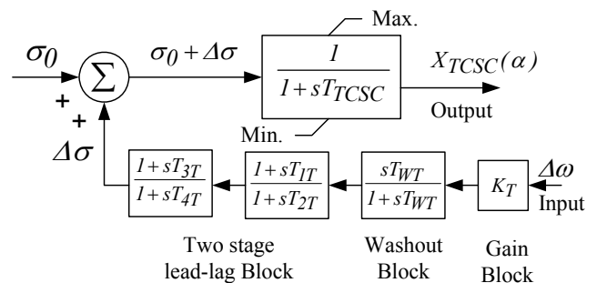
Fig. 3 Structure of TCSC-based controller
