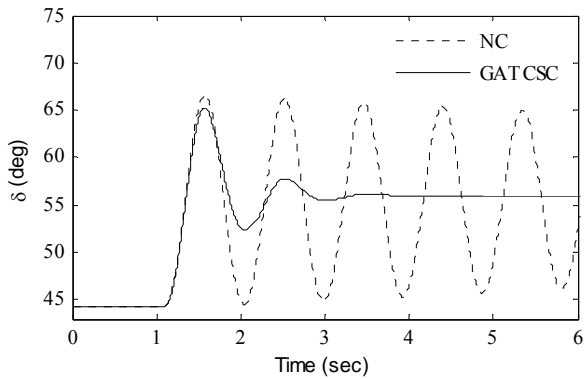
Fig. 18 Variation of power angle \delta : Case-2
