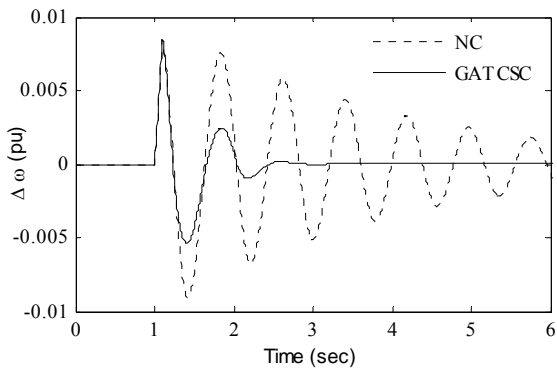
Fig. 9 Variation of speed deviation \Delta\omega : Case-1
