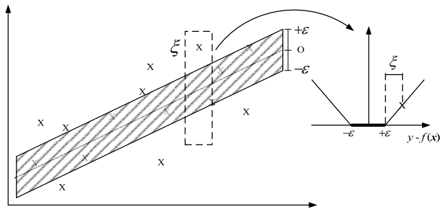
Fig. 1 The \varepsilon -insensitive loss function.
