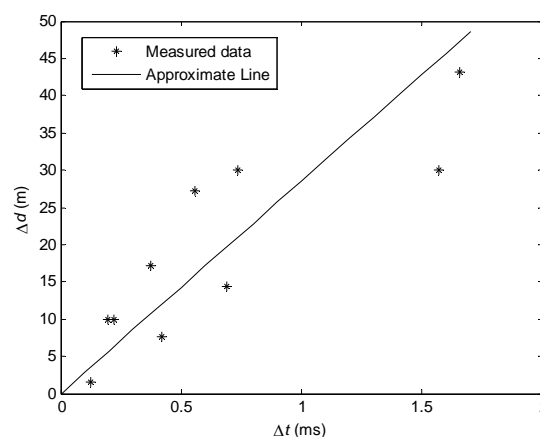
Fig. 8. The relation between time delays and distances
