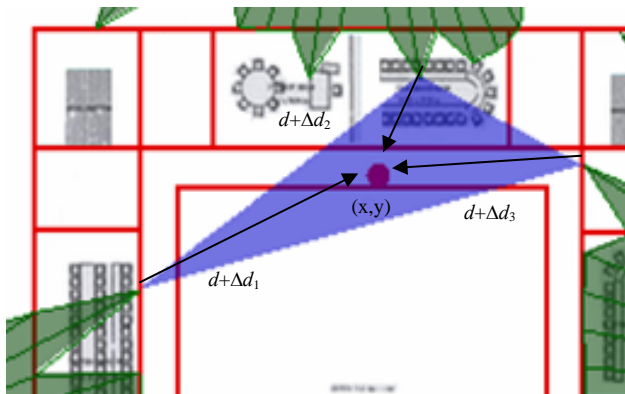
Fig. 11. Triangle locating of joint RSS and TOA
