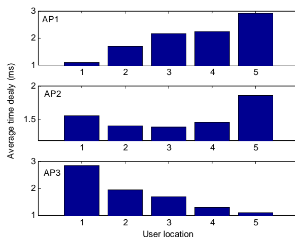
Fig. 7. The average delay time versus user location
