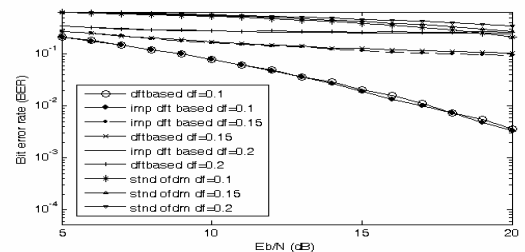
Fig. 7 BER vs E_b/N plot for standard OFDM, DFT-based scheme, and proposed scheme at \varepsilon = 0.1, \varepsilon = 0.15, \varepsilon = 0.2
