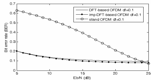
Fig. 6 BER vs E_b/N plot for standard OFDM, DFT-based scheme, and proposed scheme at \varepsilon = 0.1
