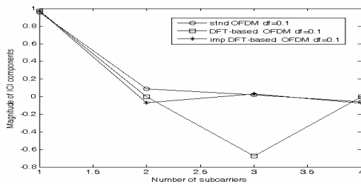
Fig. 3 Magnitude of ICI components of standard OFDM, DFT-based, and proposed schemes at \varepsilon = 0.1
