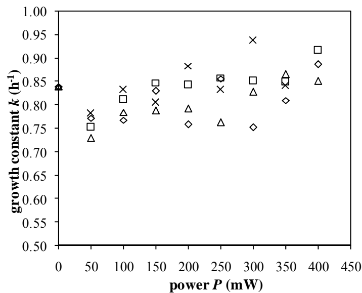
Fig. 3 Experimental values of the growth constant as a function of power and frequency of the radiation ( \diamond v=2.30 GHz; \square v=2.40 GHz; \Delta v=2.50 GHz; \times v=2.60 GHz).
