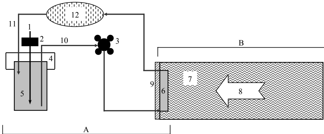
Fig. 1 Scheme of proposed experimental structure (A: sterilizable circuit; B: irradiated environment; 1: external air; 2: 20 \mu\text{m} ceramic filter for external air; 3: peristaltic pump; 4: cap; 5: Pyrex bottle containing the suspension to be irradiated; 6: PFR where the bacterial suspension is irradiated; 7: waveguide; 8: incident radiation; 9: PFR supporting plate positioned as the waveguide closure ; 10: extraction of the bacterial suspension from bottle; 11: recycling of the bacterial suspension to the bottle; 12: continuous system of spectrophotometric analysis)
