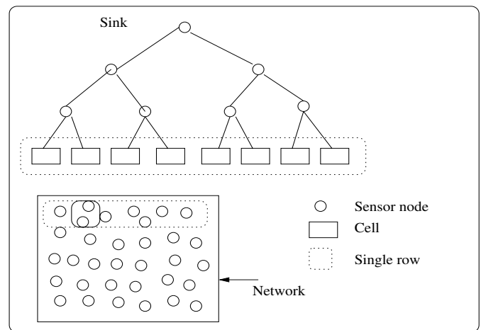
Fig. 1: The ToD construction from one row's point of view.
