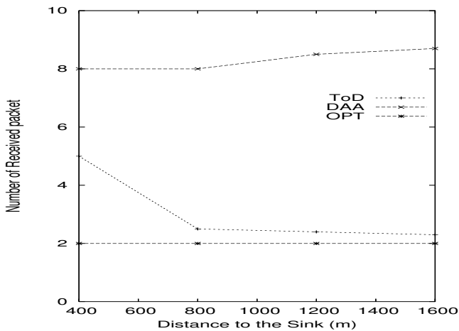
Fig. 8: Number of received packets.
