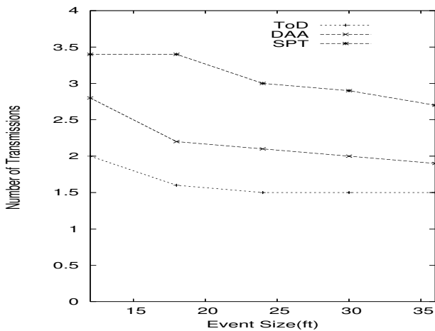
Fig. 4: The normalized number of transmissions for different event sizes.
