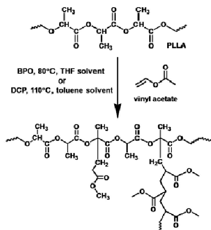
Fig. 1 Synthesis route to poly(lactide)-g-poly(vinyl acetate)
