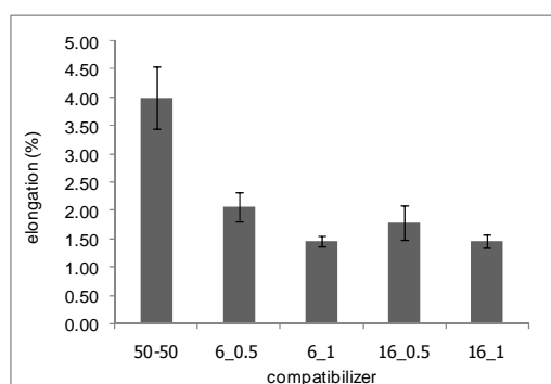
Fig. 4 Mechanical properties of starch / PLLA blend with and without PLLA-g-PVAc compatibilizer
