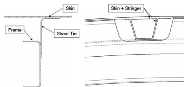
Fig. 7 Section view of composite skin panel attachments
