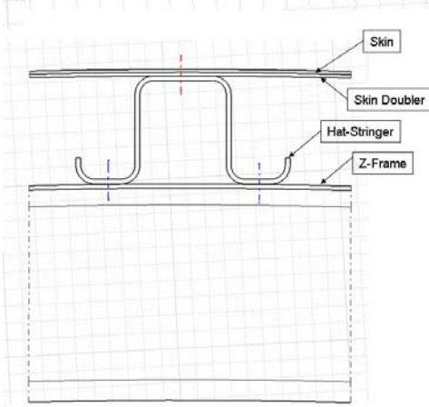
Fig. 2 Section view of metallic skin panel attachments
