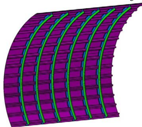
Fig. 6 CAD Model of Composite skin panel
