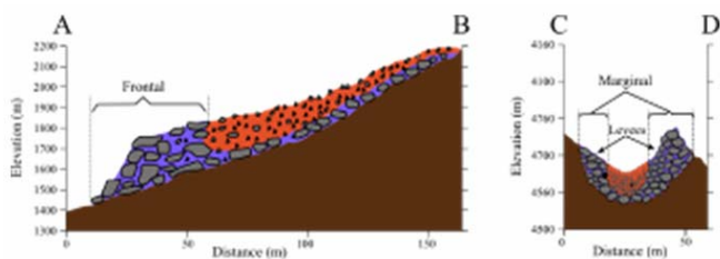
Fig. 8 Simplified vertical cross-section of the P-zone along A-B and C-D lines in Fig. 6 showing variation of grain size with distance and elevation
