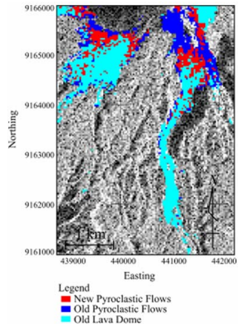
Fig. 7 Spectral Angle Mapper (SAM) classification result showing distribution of three different rock types overlaid on RADARSAT-1 \beta data after geo-referencing
