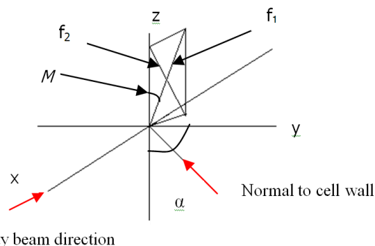
Fig. 1 Diagram showing the relationship between a cell wall, the two S_2 microfibrils and the direction of the X-ray beam [2]
