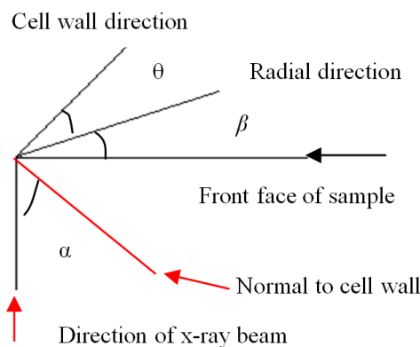
Fig. 2 Diagram showing the relation between front face of the thin sample, the radial direction ( \beta ), the cell-wall direction ( \theta ) and the direction of the X-ray beam normal to the face of sample [2]
