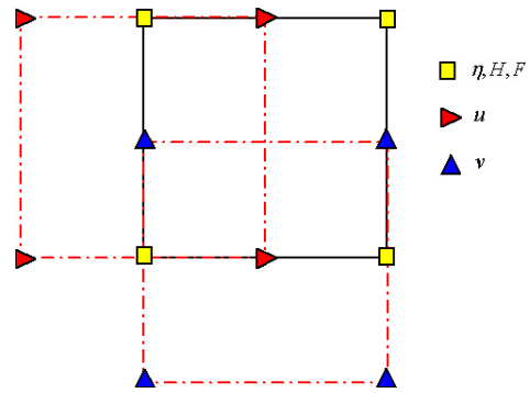
Fig. 1. Staggered C-type grid used by the hydrodynamic model. The wave model uses a nonstaggered A-type grid, in such a way that the governing equation for the wave evolution is computed at points corresponding to elevation values in the hydrodynamic model.
