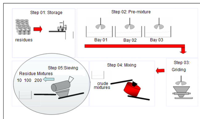
Fig. 3 Co-processing diagram
