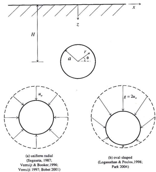
Fig. 2 Ground deformation patterns around the tunnel section
