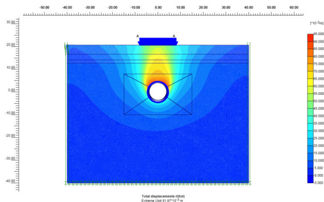
Fig. 5 Calculated total displacement
