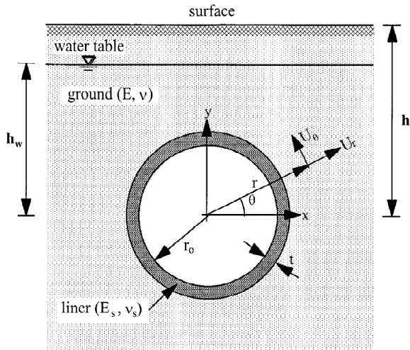
Fig. 1 Shallow tunnel
