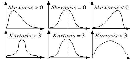
Fig. 4 Skewness and Kurtosis
