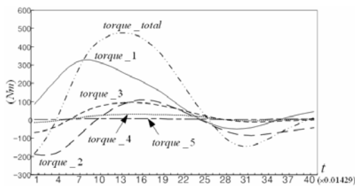
Fig. 10 Human Torque
