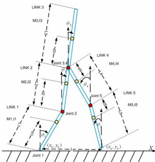
Fig. 2 5-link biped model
