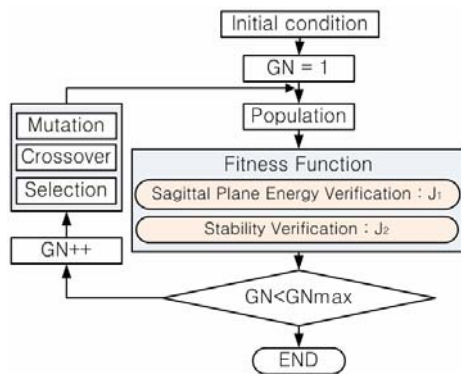
Fig. 7 Genetic Algorithm
