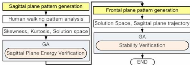
Fig. 6 Adaptive walking pattern generator
