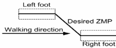
Fig. 5 Desired ZMP
