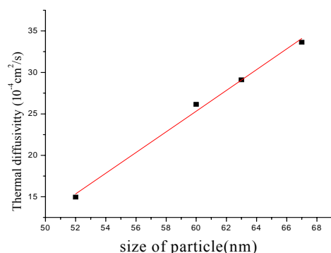
Fig. 5 Thermal diffusivity in term of particles size
