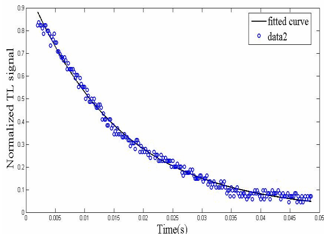
Fig. 4 The Time evolution of the TL signal for CdS nanoparticles prepared at 30 kGy dose. Solid line corresponds to the best fit of Eq. (1) to the TL experimental data
