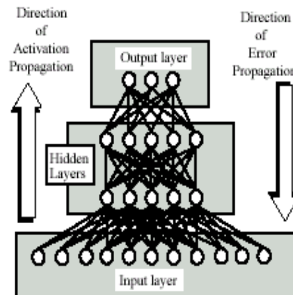
Fig. 2 Multilayer Perception
