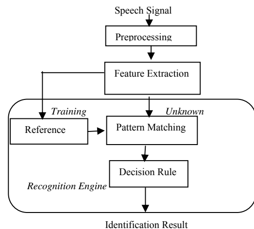
Fig. 1 Speaker Identification Model
