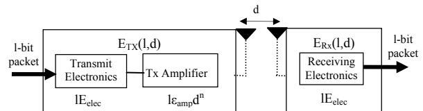
Fig. 2 Radio energy dissipation model
