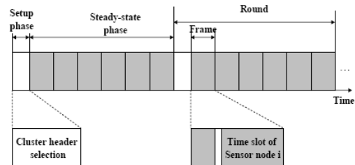
Fig. 1 Time line showing operation of LEACH
