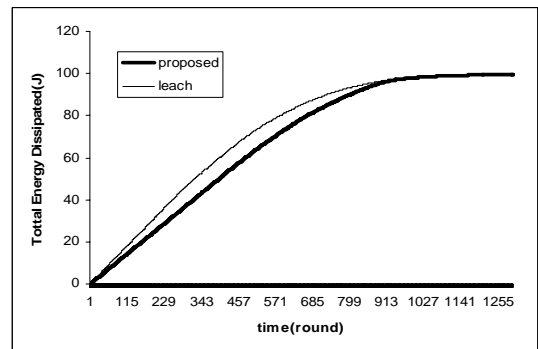
Fig. 4 Total energy dissipated in LEACH and our scheme in the first experiment
