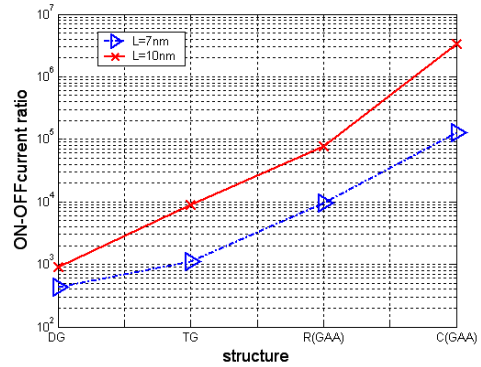
Fig. 3 I ON /I OFF ratio for different channel length of various SN T
