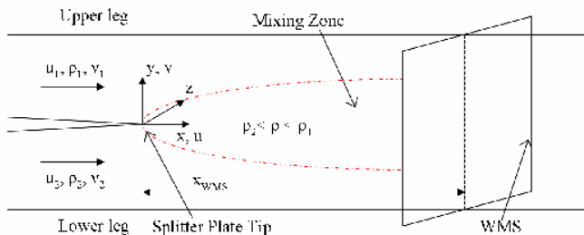
Fig. 1 Principal Sketch of GEMIX-Facility primary components
