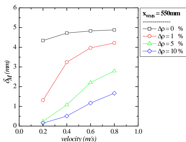
Fig. 12 The mixedness thickness \delta_M is judged as a function of velocity. The differences with fig. 6 are notable
