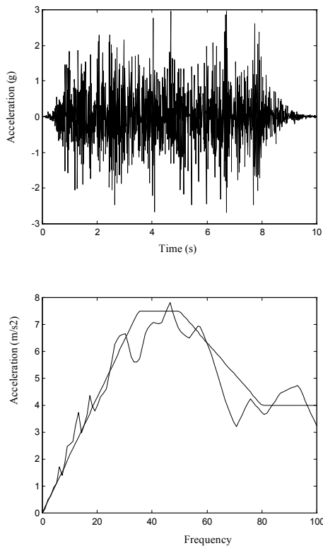
Fig. 2 Generated acceleration time history and the GRS
