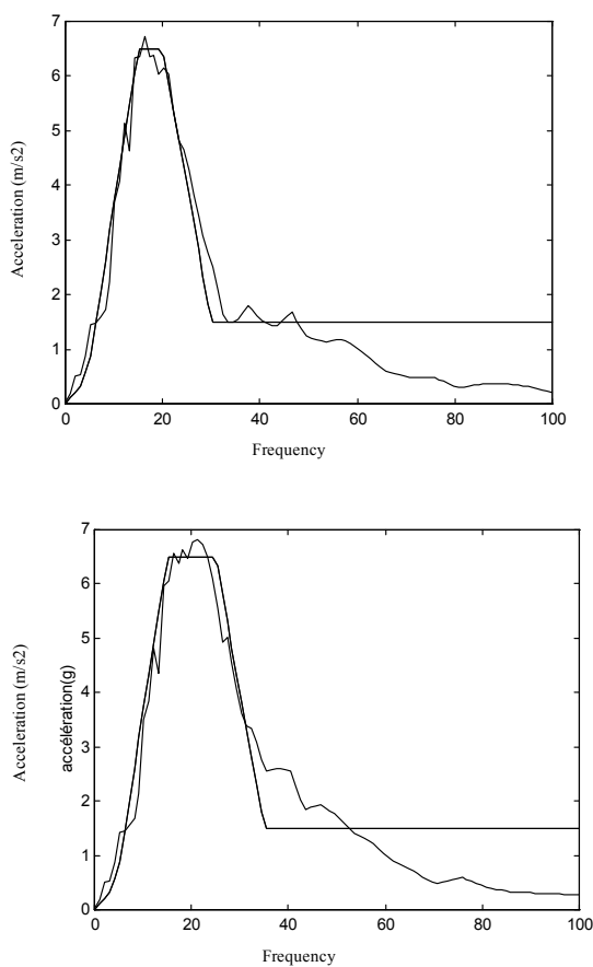
Fig. 4 Spectrum transformation of large and narrow band
