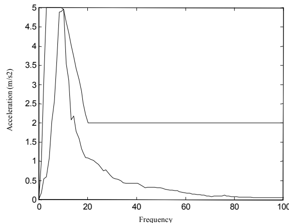
Fig. 6 Spectrum transformation at low frequency range
