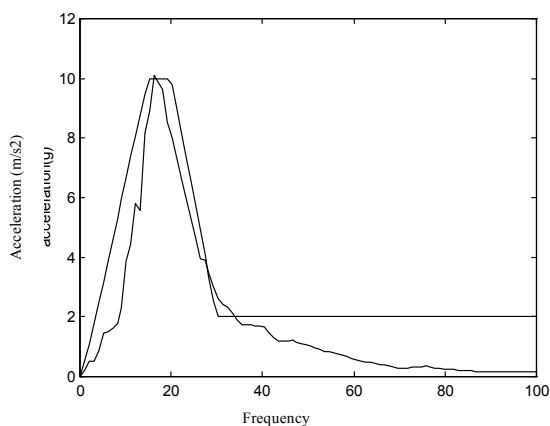
Fig. 5 Spectrum transformation of high amplification ratios RRS/GRS
