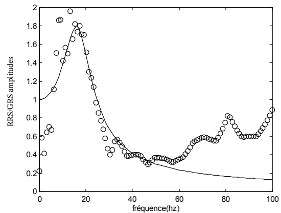
Fig. 3 Curve fitting of the amplitude ratios RRS/GRS
