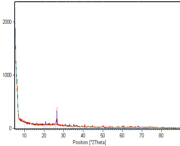
Fig. 6 XRD analysis of Catalagzi fly ash
