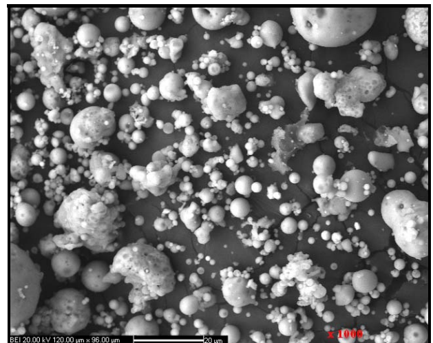
Fig. 9 SEM analysis of Catalagzi fly ash
