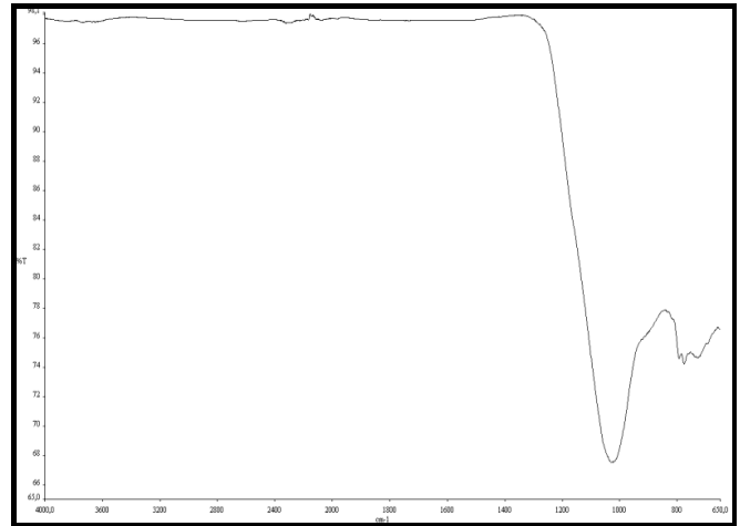
Fig. 12 FT-IR analysis of Catalagzi fly ash
