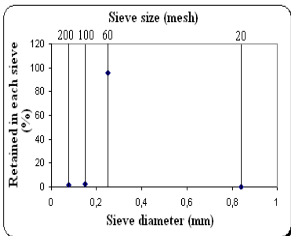
Fig. 11 Sieve analysis of Catalagzi fly ash
