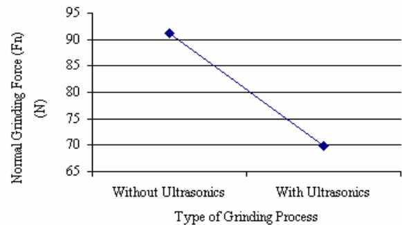
Fig. 3 Ultrasonic vibration effect on the reduction of normal grinding force
