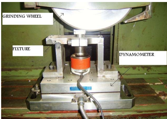
Fig. 2 Illustration of the experimental equipment
