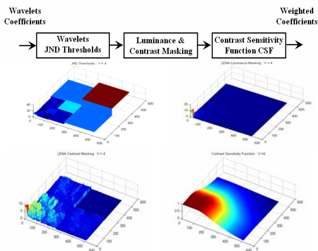
Fig. 4 Perceptual masking model SetUp
