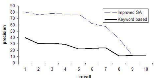
Fig. 2 Comparing improved SA with keyword search
