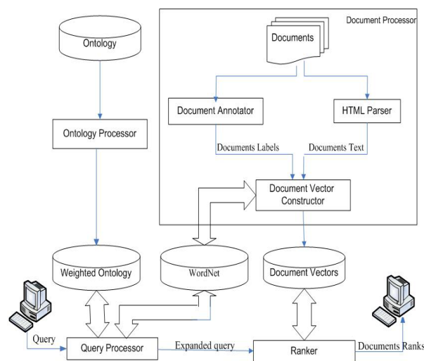
Fig.1 The structure of ORank system
