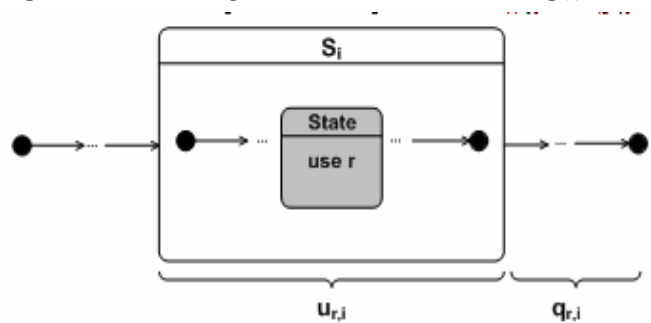
Fig. 1: The probabilities u_r(i) and q_r(i)
