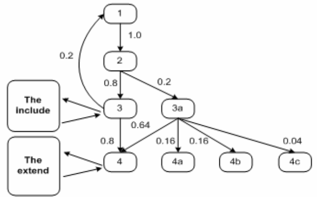
Fig. 6: The graph of the base use case.
