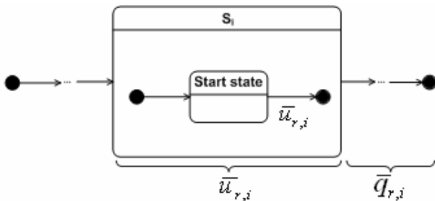
Fig. 2: The simplified service effect specification.
