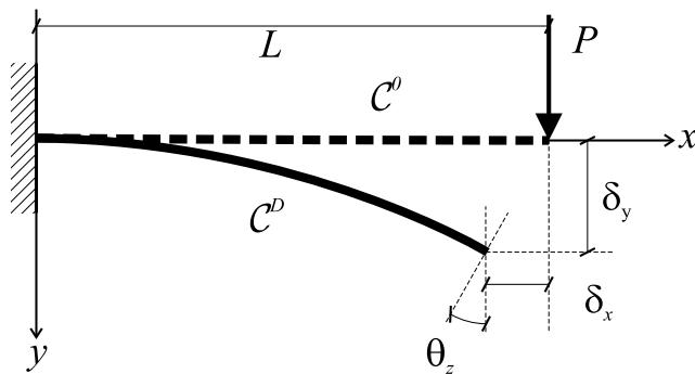
Fig. 1. Long deflection cantilever beam problem for flexible modelling
