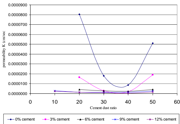
Fig. 8 permeability of sand with different cement, cement-dust ratios
