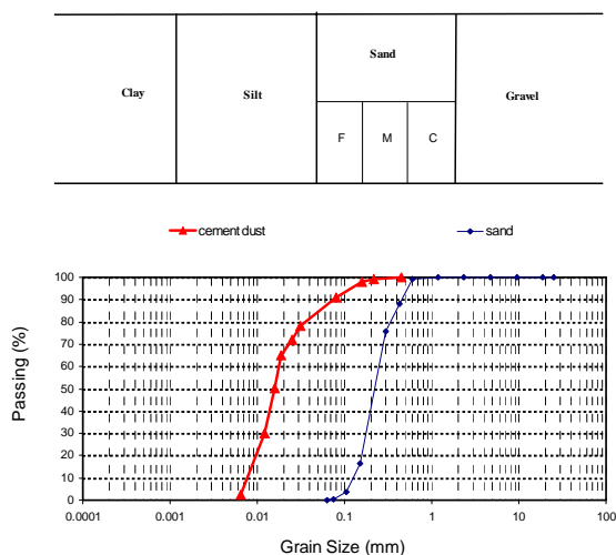
Fig. 1 Grain size distribution for the used materials
