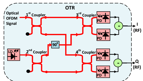
Fig. 4 Direct down-converter built for simulation
