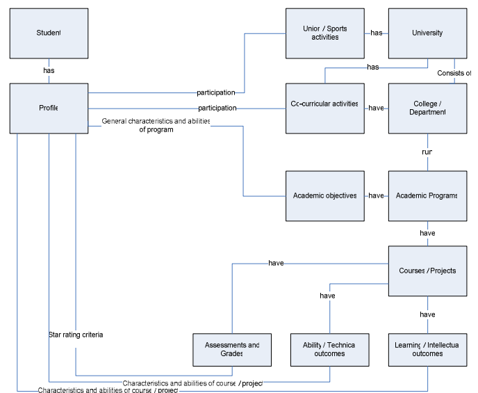
Fig. 3: Ontology Specification to develop student profiles
