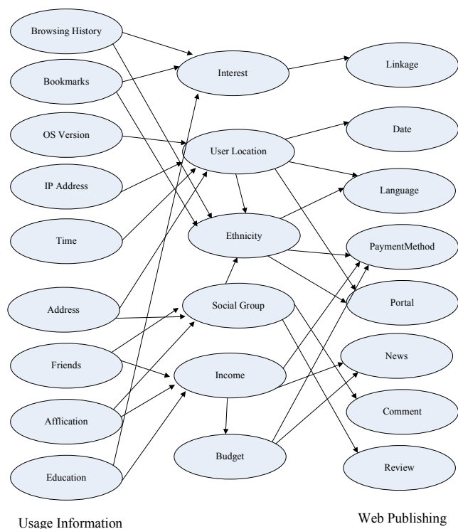
Fig. 4 Bayesian network structure
