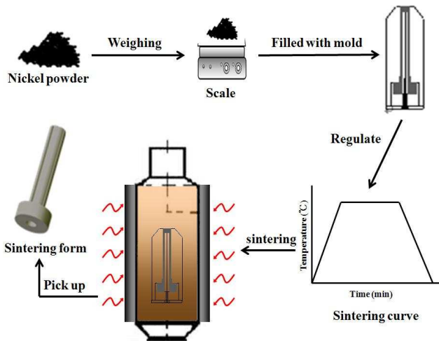
Fig. 2 Wick manufacture
