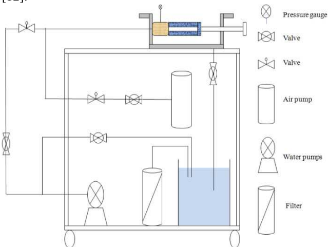
Fig. 4 Device for measuring internal parameters of wick
