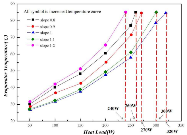
Fig. 7 Relationship between evaporator temperature and heat load
