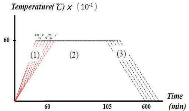
Fig. 3 Typical temperature curve
