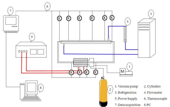
Fig. 5 Device for thermal testing of LHP
