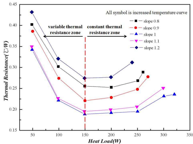
Fig. 8 Relationship between thermal resistance and heat load
